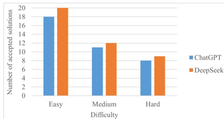
Fig. 3. The number of accepted solutions by difficulty categories for the ChatGPT-4o and DeepSeek V3 models
